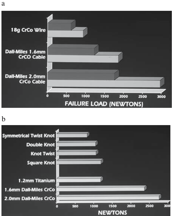
FIG. 2. a Comparative strength of fastening methods ( darker bars ) and cerclage material ( lighter bars ). b Comparative strengths of various wire fastening methods ( top, darker bars ) and cable fastening methods ( bottom, lighter bars )
